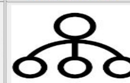
Distribution
