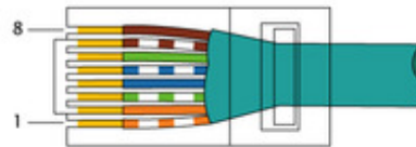
EIA/TIA-568B
