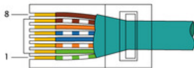
EIA/TIA-568A
