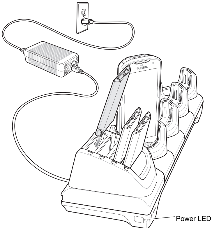
Figure 146 Spare Battery Charging
