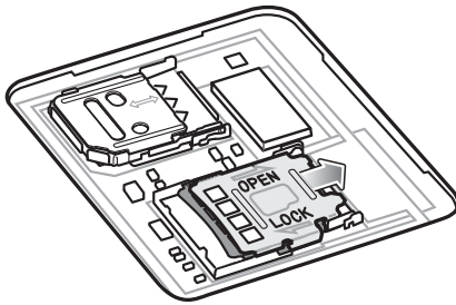
Figure 11 Unlock microSD Card Holder
