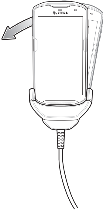
Figure 170 Rotate Device into Cable Cup
