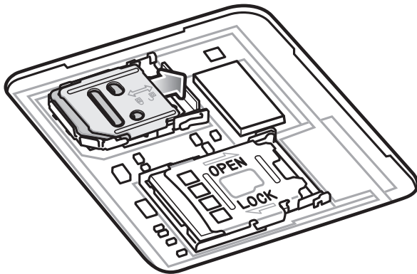
Figure 23 Unlock SIM Card Door
