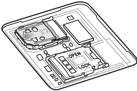
Figure 8 Lock SIM Card Holder Door
