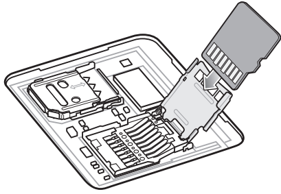
Figure 13 Insert microSD Card in Holder
