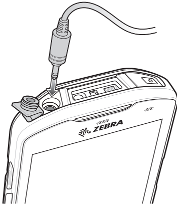
Figure 49 3.5 mm Headset Adapter
