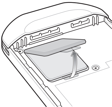
Figure 3 Remove Access Door
