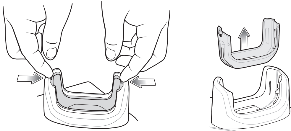
Figure 147 Remove Insert from Cup
