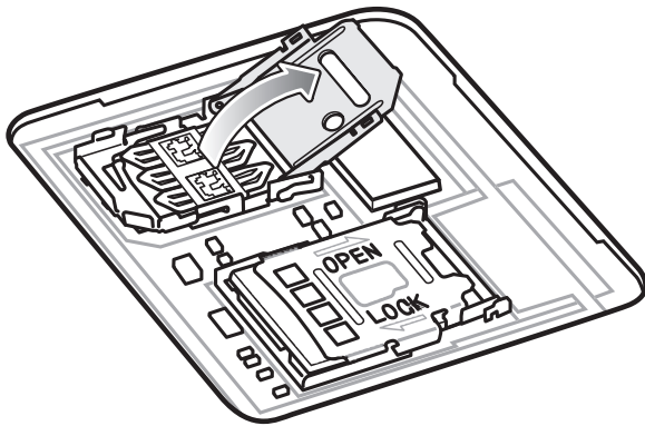
Figure 5 Lift the SIM Card Holder
