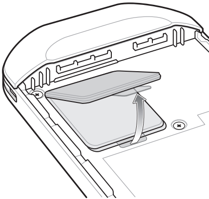
Figure 10 Lift Access Door
