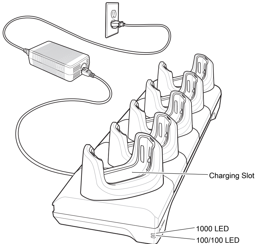
Figure 151 5-Slot Ethernet Cradle
