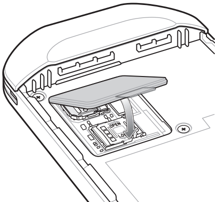
Figure 9 Replace Access Door
