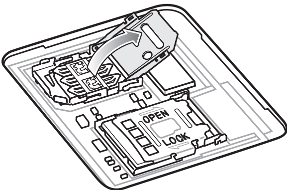
Figure 24 Lift the SIM Card Door
