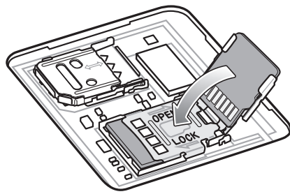
Figure 14 Re-install Access Door
